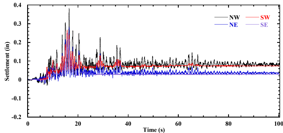
Bridge Seat Settlement Measurements at Corners
