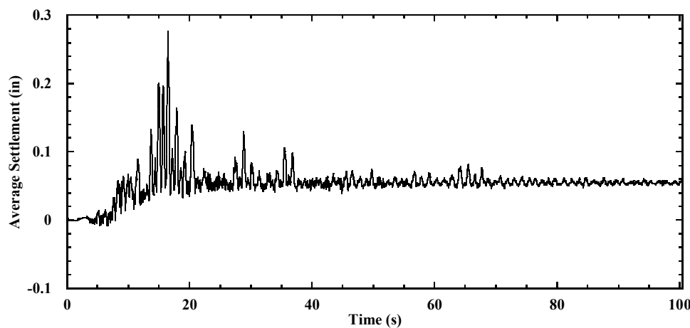
Average Bridge Seat Settlement
