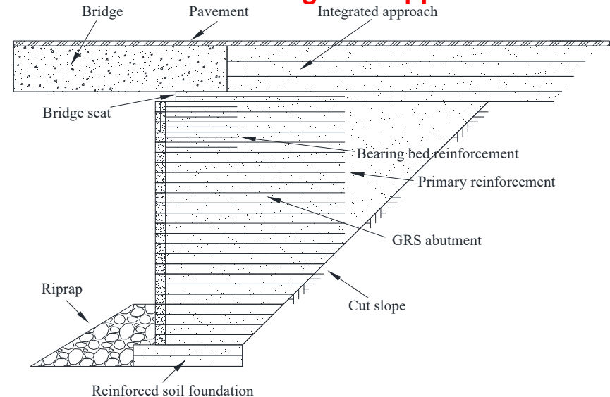
GRS-IBS Abutment
